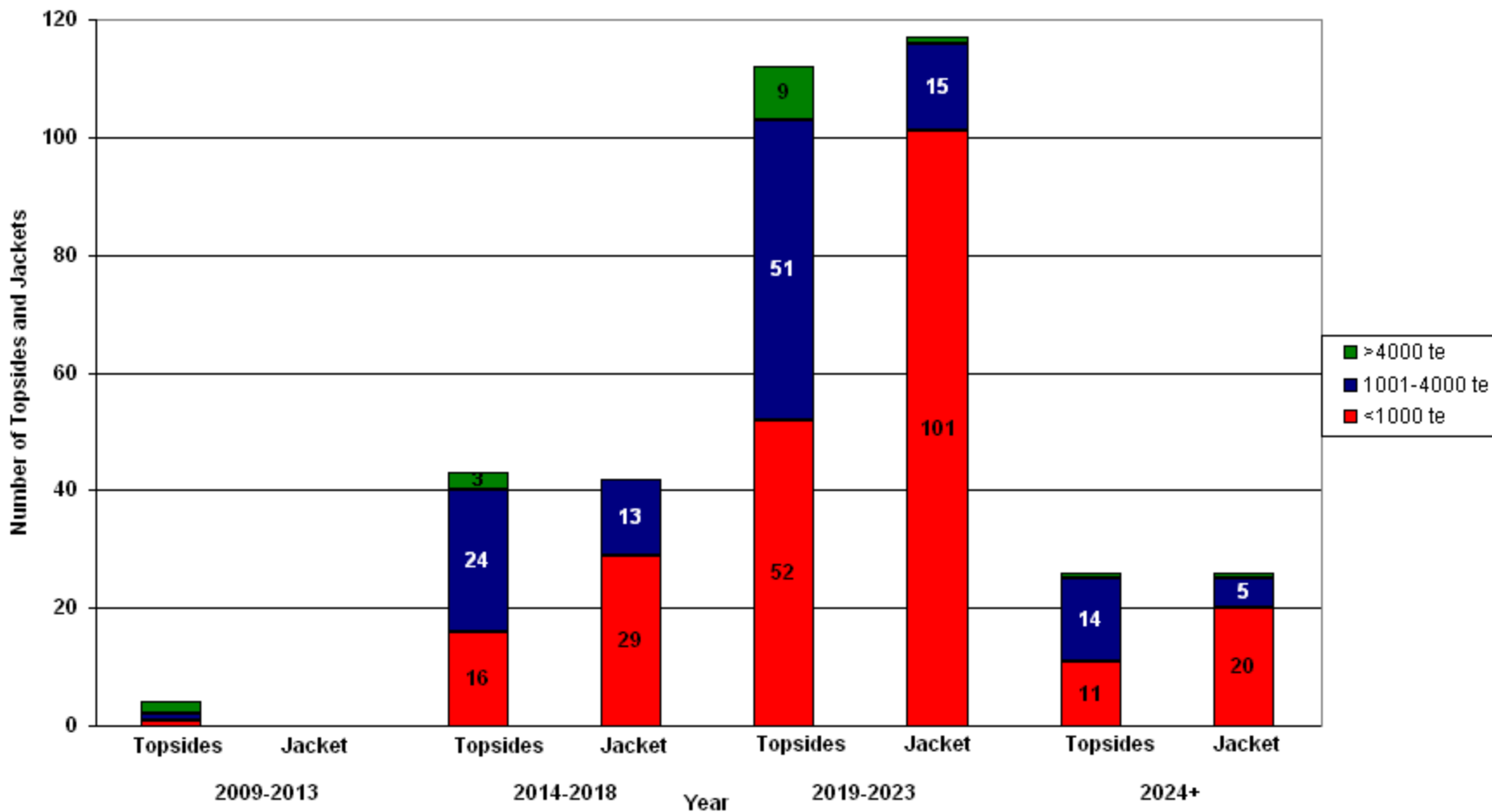
Number of Topsides and Jackets to be Decommissioned by weight category SNS UK Sector
